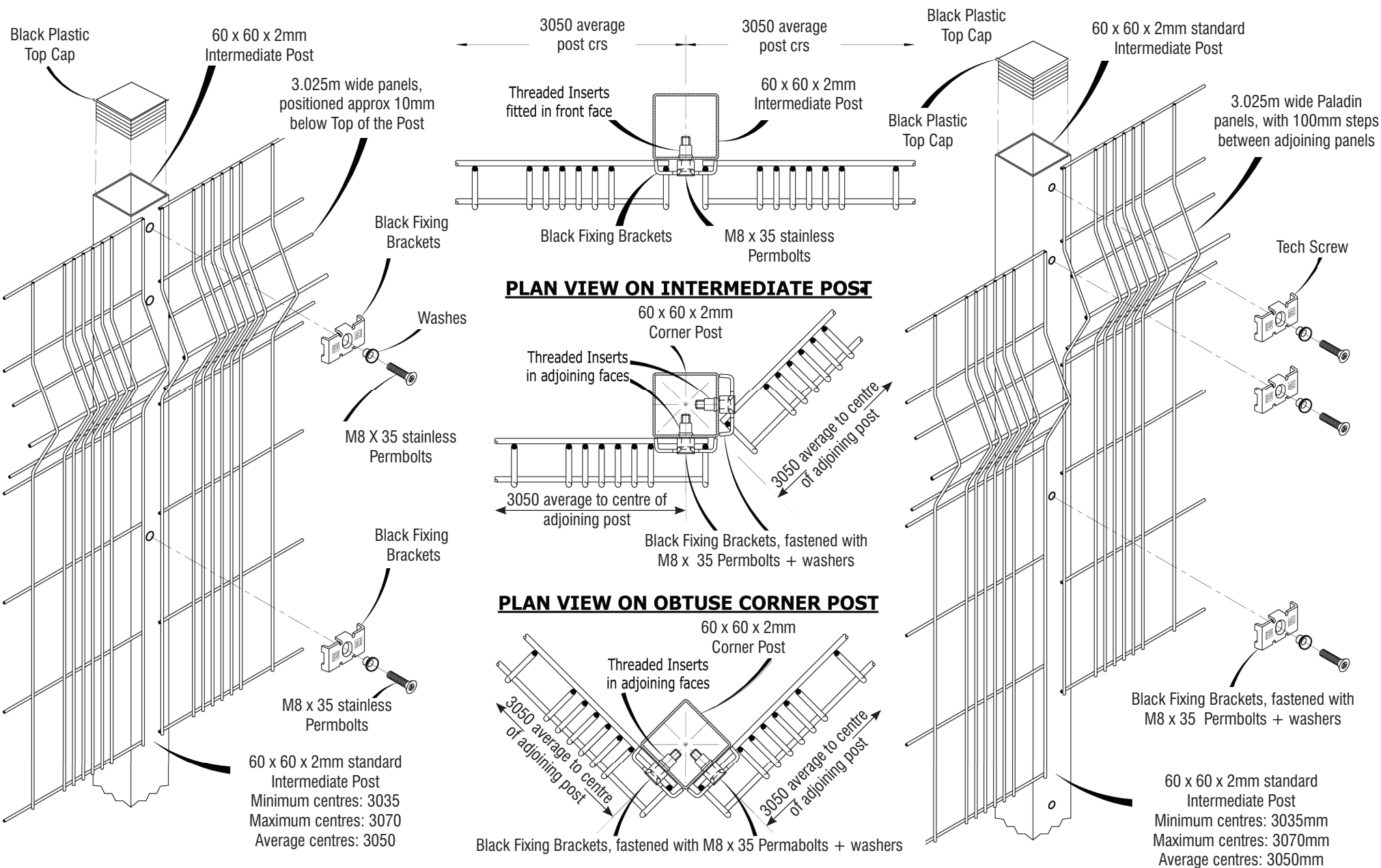
TYPICAL POST AND PANEL FIXING DETAILS FOR LEVEL GROUND
